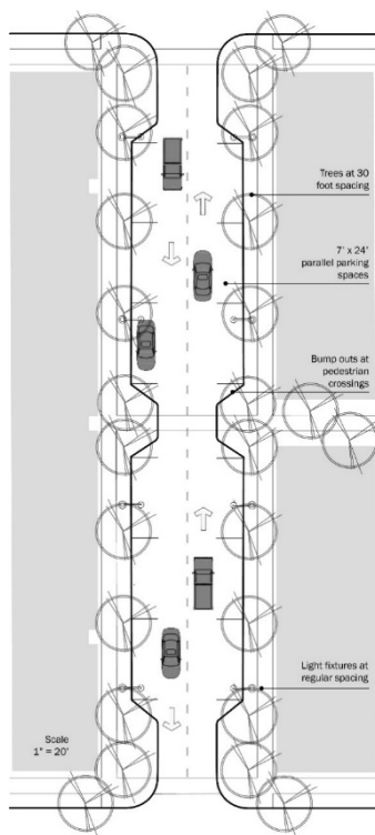
Fig. A.1.S5.a: Plan view diagram of Primary Internal Drive showing optional parallel parking.
